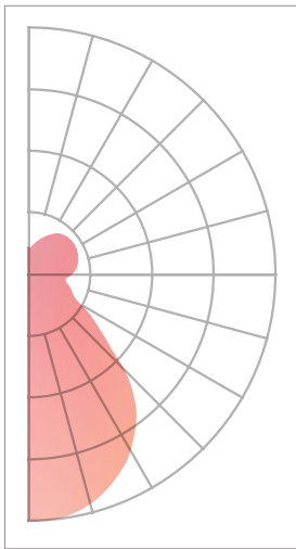
935 HE – High Efficiency at 0° Vertical
